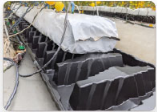
One piece base for even drainage into build-in gutter.
